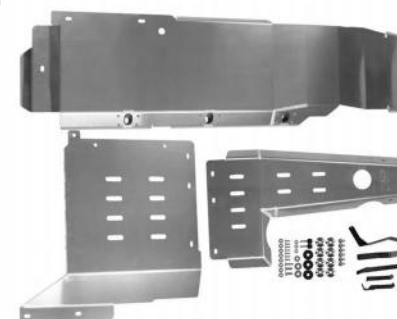
JL lower guard plate (aluminium)
